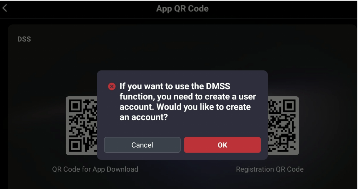
Figure 4-11 Onscreen prompt
